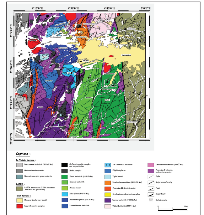
Geological map of the study area (Bechiri et al., 2003) and stations of magnetotelluric survey
