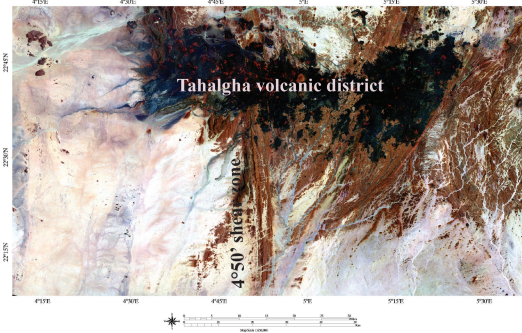
RGB 5 (90-45-135) (Kavak et Cetin 2007) color composite image with convolution of 7X7 RGB (7-5-3) False color composite image for study area
