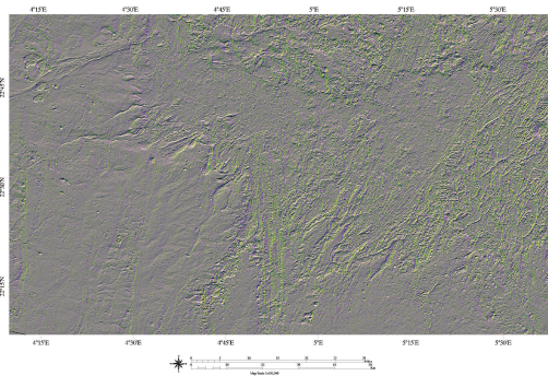
RGB 5 (90-45-135) (Kavak et Cetin 2007) color composite image with convolution of 7X7 RGB (7-5-3) False color composite image for study area
